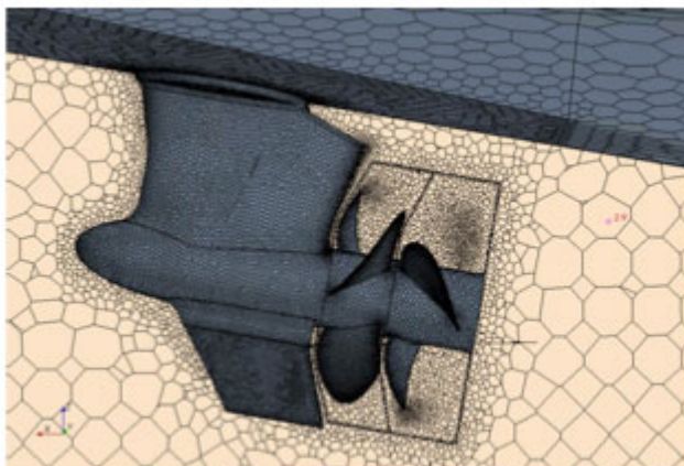
Figure 21. CFD mesh in the region of the pod system
